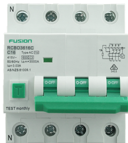
RCBO3620C
